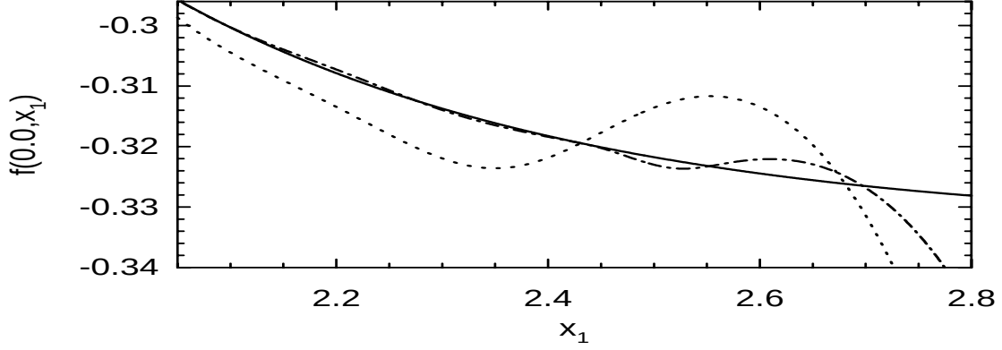
Figure 18: A one-dimensional slice at x = 0 of a two dimensional delay embedding of the Stiletto Map. The one step ahead prediction f(x_0, x_1) is shown for x_0 = 0 as a function of x_1 for the perfect model (solid) and two global RBF models using 64 centers (dotted) and 128 centers (dash-dotted).
